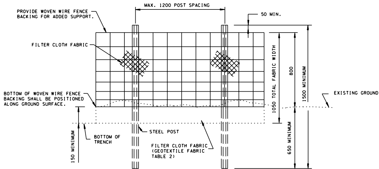
ELEVATION VIEW
