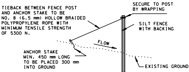
SILT FENCE TIEBACK
