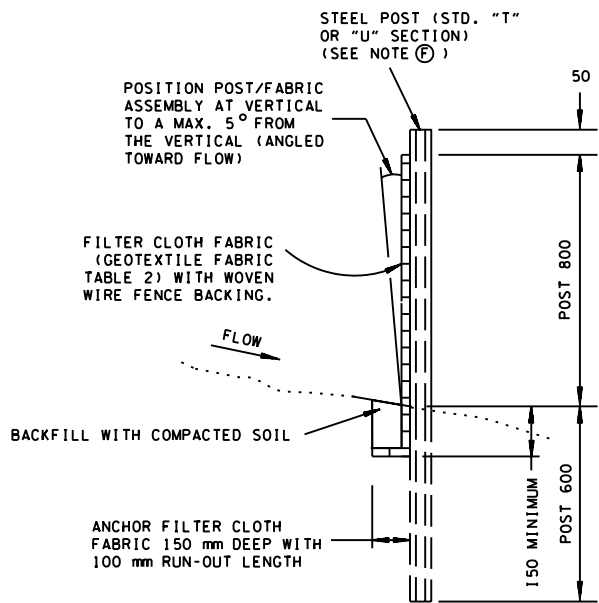
SECTIONAL VIEW
